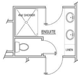
UNIT 'A' OPTIONAL ENSUITE FLOOR PLAN SCALE 1/4" = 1'-0"
