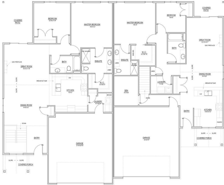
UNIT 'A' FLOOR PLAN 1,515 SQ. FT. (+ 538 SQ. FT. GARAGE)
